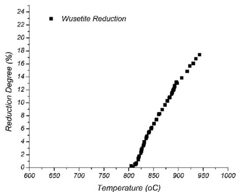
Fig. 10(a) Reduction of magnetite by VM.(b)Reduction of wüstite by VM
