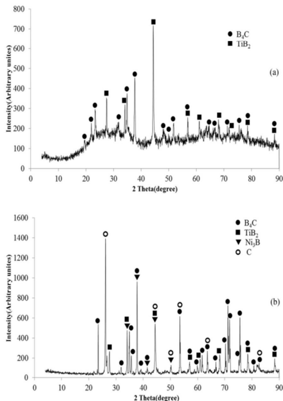
Fig. 3. X-ray diffraction analysis of N5 sample before (a) and after (b) sintering at 2175^\circ C .
