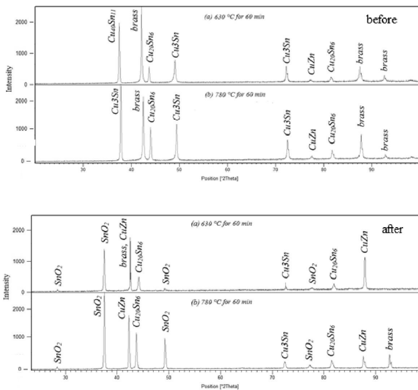
Fig. 9. XRD patterns of annealed ADB before and after ten days exposure to 3.5%NaCl solution: (a) 630°C for 60min) 780°C for 60min.
