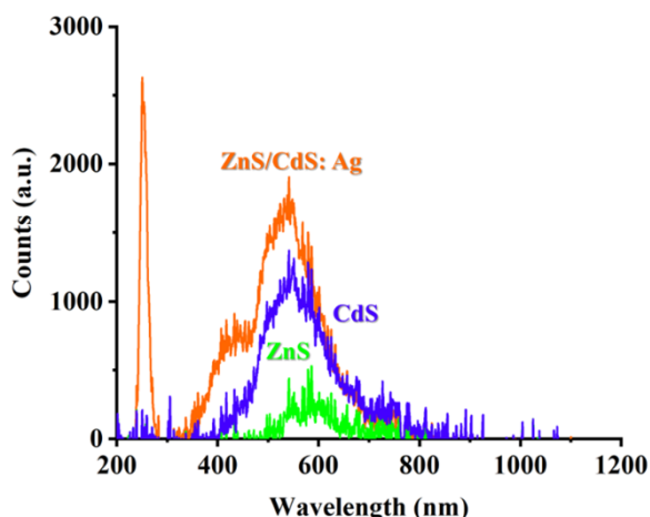
Fig. 7. IBIL spectrum of pure samples and Ag-doped ZnS/CdS nanocomposite
