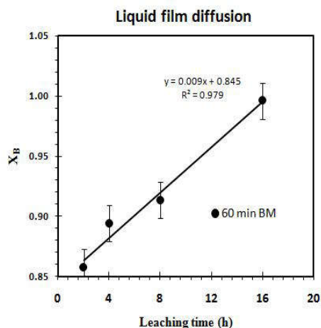
Fig. 9. Plot of the liquid film diffusion equation between 2-16 h for sample 60BM.
