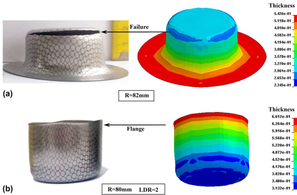
Fig. 6. Rupture loci and thickness distribution based on FE simulation in the deep drawn cup from circular blanks diameter of (a) 82 mm and (b) 80 mm under optimum condition
