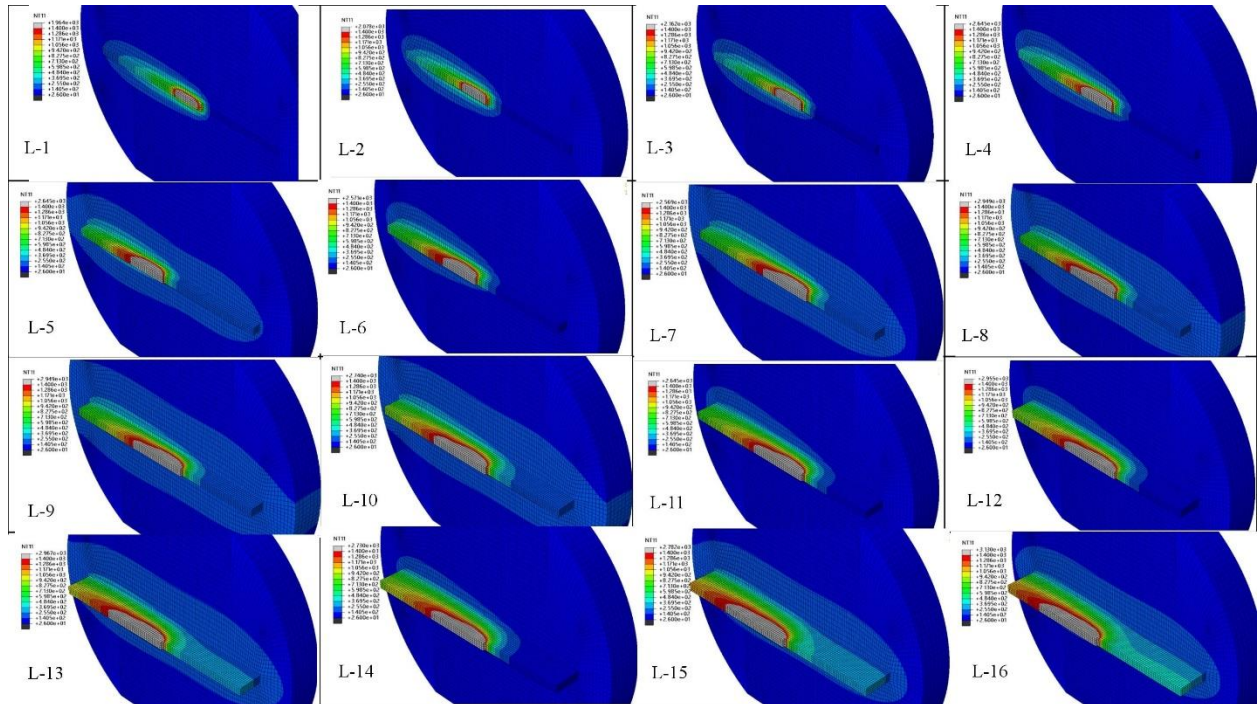
Figure 5. Temperature distribution across 16 deposited layers
