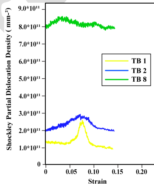
Fig. 4. Evolution of dislocation density with strain in the TB1, TB2, and TB8 models.
