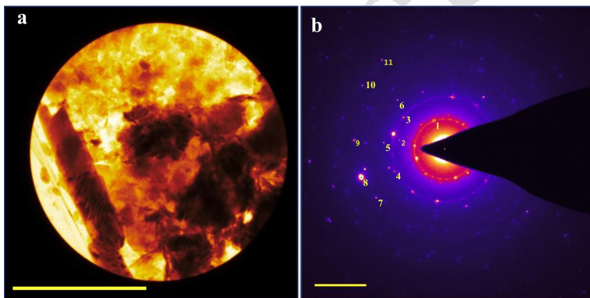
Fig.9. a) and b) TEM and SAED pattern of another region of GCNP sample, respectively. The SAED pattern of (a) comprises of spots, narrow ring and a diffused circle in the centre, indicating the composite nature of the area including large crystals, polycrystalline area and amorphous regions, respectively. Crystalline planes attributed to spots and rings are listed in Table 5.
