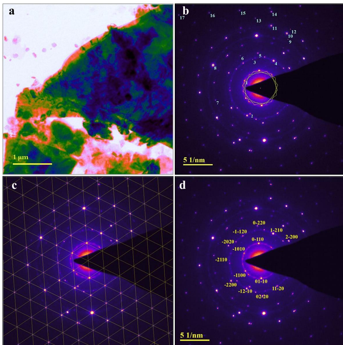
Figure 3. a) TEM image of GCNP consisting of large multilayer particles besides small hexagonal flakes (upper left of the image, restricted in a small rectangular). b) SAED pattern of the TEM image(a), composed of a significant number of diffraction spots covering all the entire pattern and a few narrow circles. This pattern is attributed to the existence indicates the presence of crystalline areas with large sizes as well as polycrystalline areas. The hexagonal arrangement of spots shows a p6mm symmetry of the crystals. The related crystalline planes according to d-spacings calculated from the radius of spots are presented in Table 2. Three hexagons in the central part of the pattern show the presence of at least three crystalline layers in the studied region. c) The SAED pattern meshed by parallel lines with a 60^\circ angle passing through the spots of the pattern, showing the exceptionally highly ordered structure of the sample. d) The indexed SAED pattern obtained from solving the hexagonal crystal lattice.
