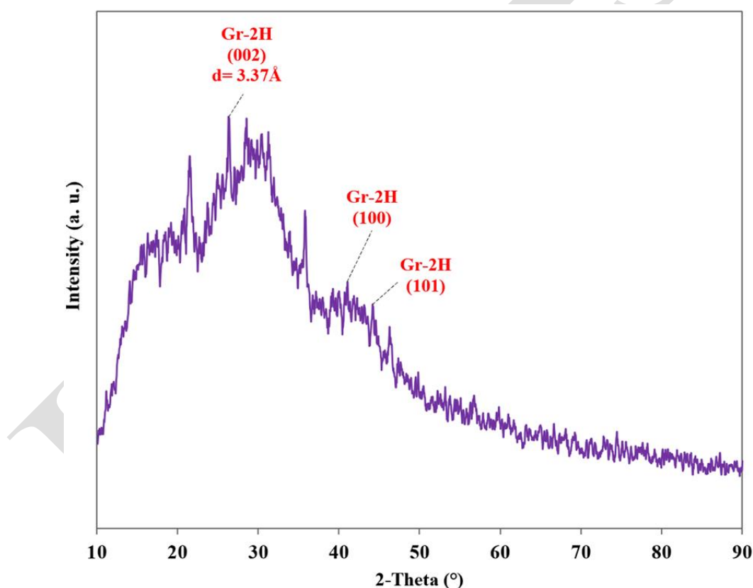
Figure 2. XRD pattern of GCNP sample representing indicating the composite nature of the material consisting of crystalline and amorphous phases. The inset shows the comparison of the sample peaks with Graphite-2H (PDF 41-1487) which matches to a high extent.
