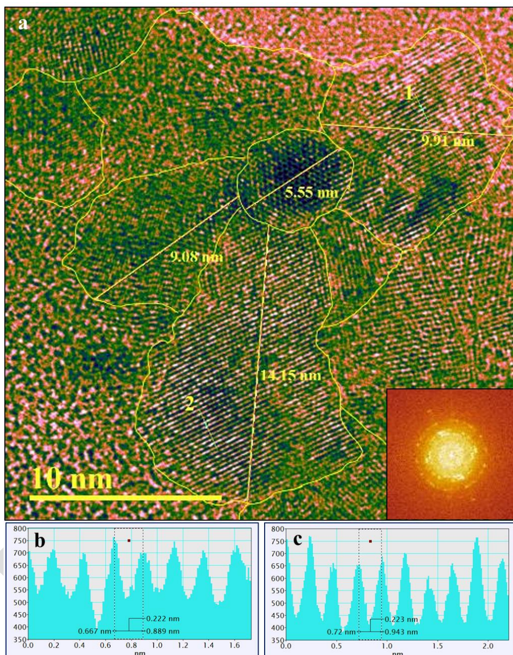
Figure 8. a) A polycrystalline area of GCNP sample with various growth directions. Some of the grain sizes are shown in the picture. The inset shows an FFT image in which multiple spots imply the presence of several crystalline domains in the studied region. Lattice fringes were measured in randomly selected regions which are displayed in b) and c). d-spacings are related to (100) crystalline plane of Graphite-2H structure according to JCPDS card 41-1487.
