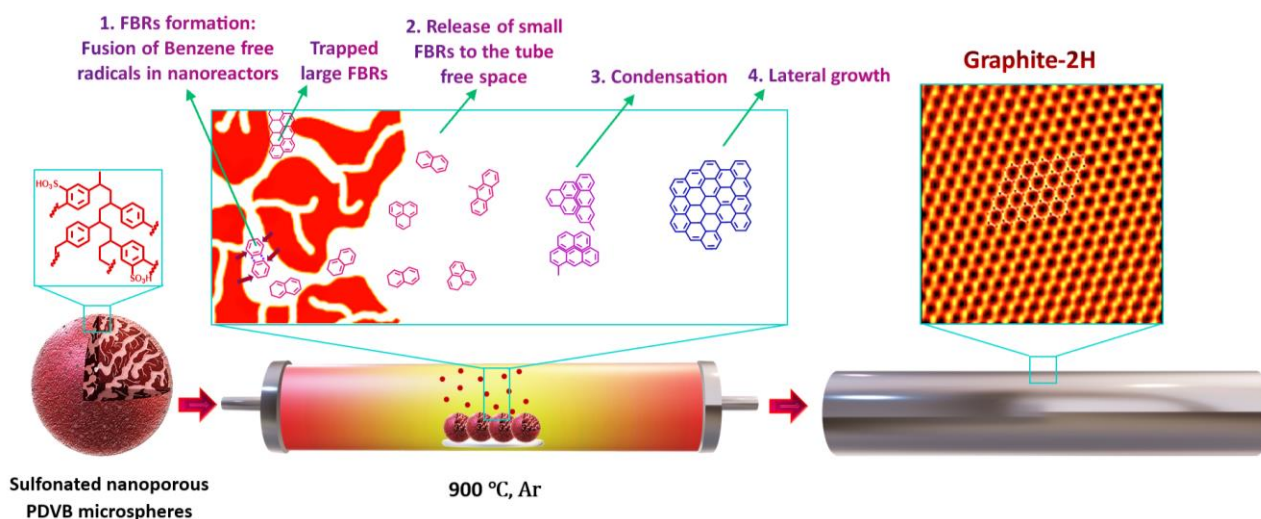
Figure 12. Schematic for the representation of the nanoreactors network-directed molecular fusion mechanism for the formation of crystalline Graphite-2H from carbonization of sulfonated nanoporous PDVB microspheres.
