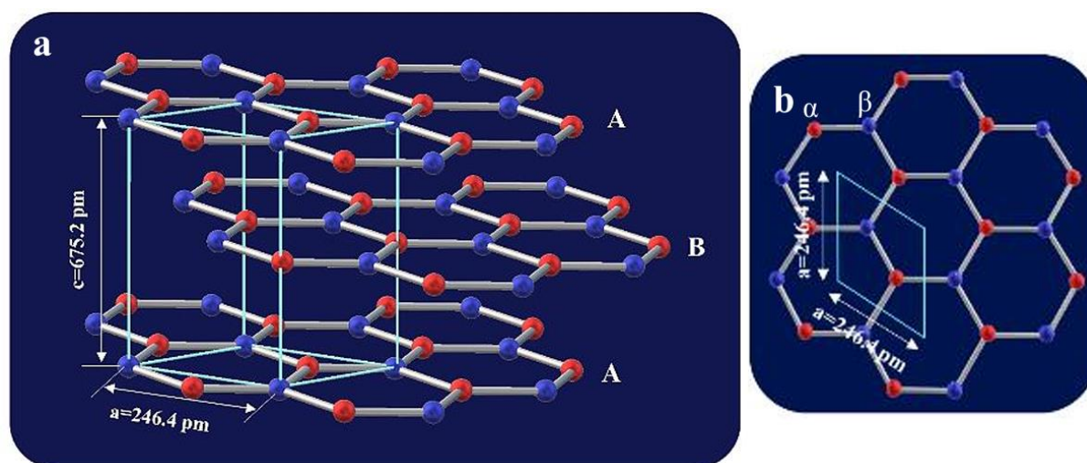
Figure 4. Constructed structure of graphite-2H according to the calculated lattice constants from SAED pattern a) Side view of the graphite structure with Bernal stacking order ABA. Red and blue spheres represent C atoms in \alpha and \beta positions sites of the Graphite basal plane (graphene layer). The corresponding unit cell is determined by a light blue rhombohedral prism. Dimensions of the prism are designed according to the lattice constants obtained from calculations of the SAED pattern, presented in Table 3. b) Top view of Graphite basal plane (a single graphene layer) in which the unit cell is displayed with a light blue rhombic shape. The lattice constant equals the calculated “a” shown in Table 3. The unit cell constants are in excellent agreement with the Graphite-2H unit cell (a lattice constant of Graphite-2H=0.246.9 pm and the c parameter of this structure is 675.2 pm).
