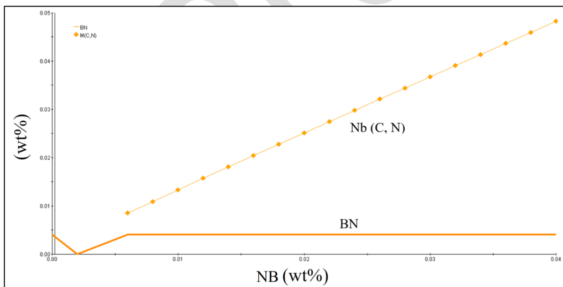
Figure 2. Effect of Nb addition on the BN content.
