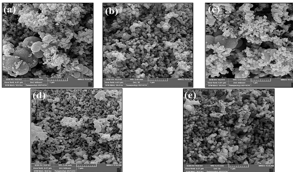
Fig. 3. The FESEM images taken from the \text{TiO}_2\text{-ZnO} nanocomposites calcinated at the times of (a) 1, (b) 1.5, (c) 2, (d) 2.5, and (e) 3 hour (s)
