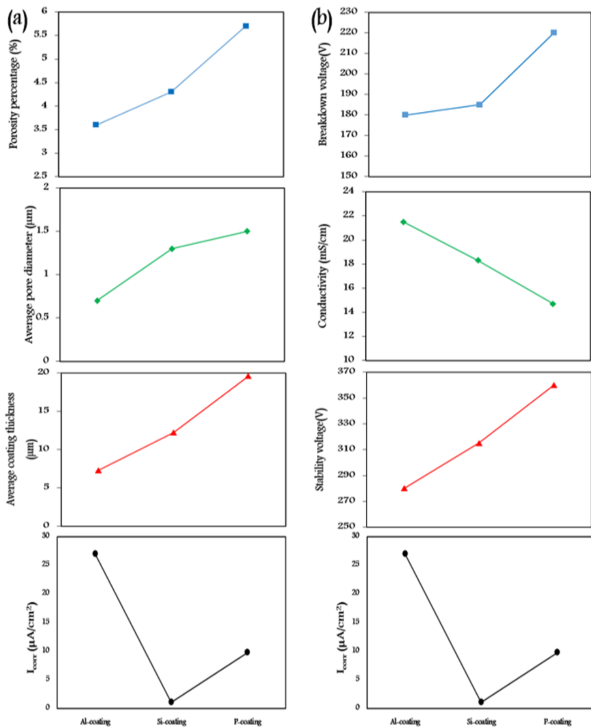
Fig.7. Correlation of i_{\text{corr}} with Morphological characteristics (a), electrical process characteristics (b) measured for coatings.
