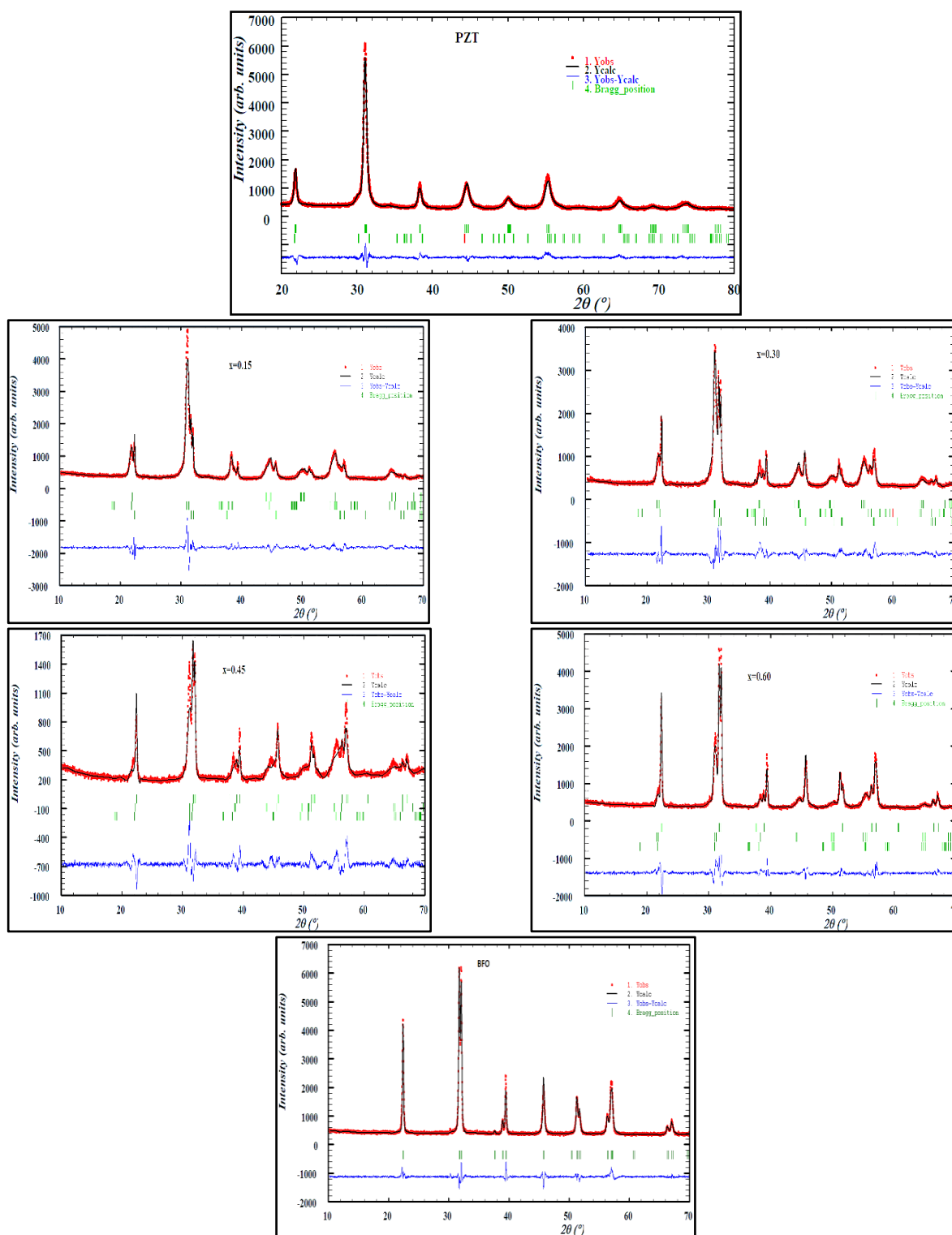
Fig. 2. Rietveld refinement of (1-x)\text{PZT-xBFO} powders
