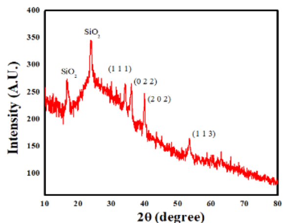
Fig. 4. XRD pattern of CuO thin films.
