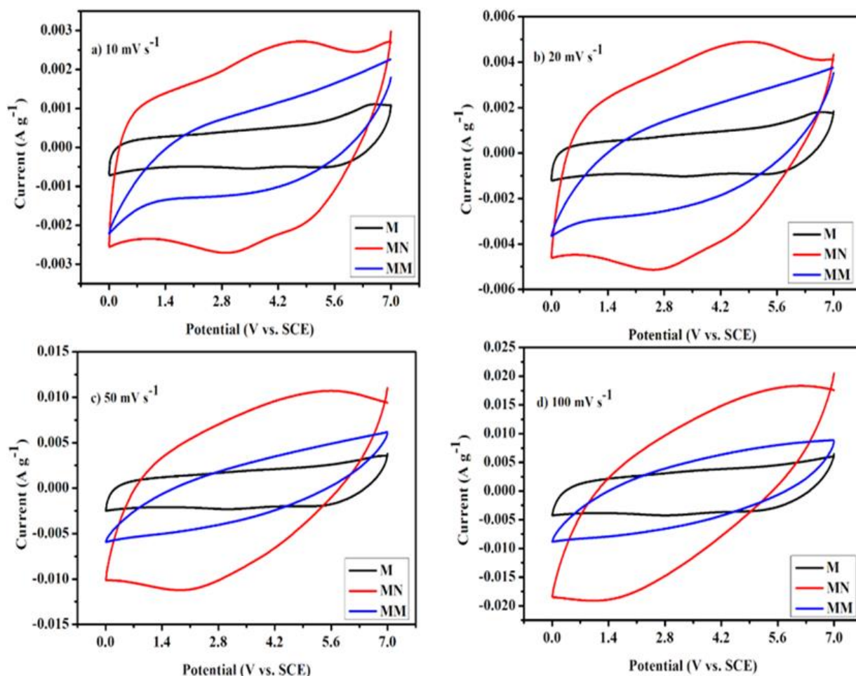
Fig. 6. The cyclic voltammograms of MN, MM, and M thin films at scan rates a) 10, b) 20, c) 50, and d) 100 \text{mV s}^{-1} .
