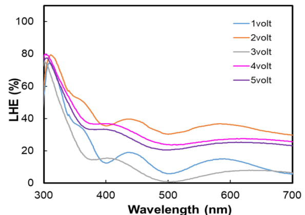
Fig. 7. Light Harvesting Efficiency (LHE)
