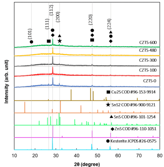
Fig. 6. XRD diffraction patterns show the formation of ZnS, \text{Cu}_2\text{S} , SnS, and \text{SnS}_2 as secondary phases
