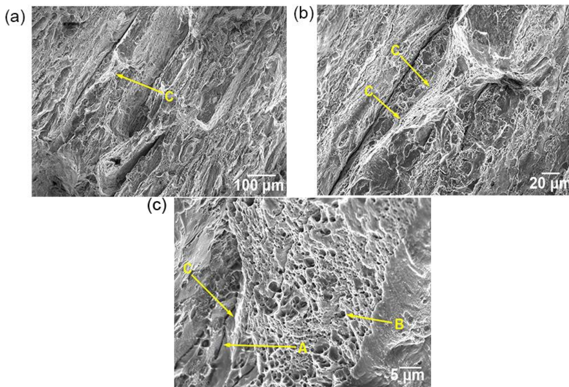
Fig. 9. Fractography of the base material at (a) 125 \times magnification; (b) 400 \times magnification; (c) 2000 \times magnification
