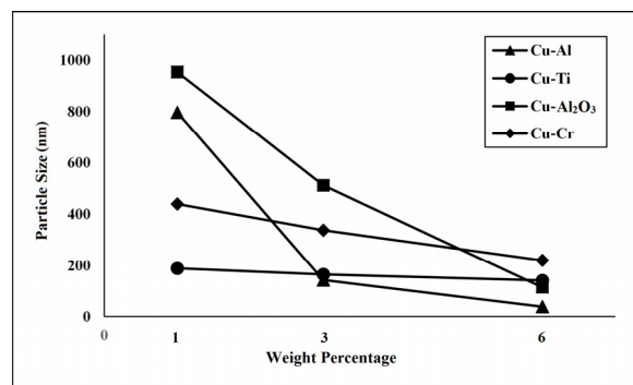
Fig. 5. Particle Size Distribution of the synthesized samples.
