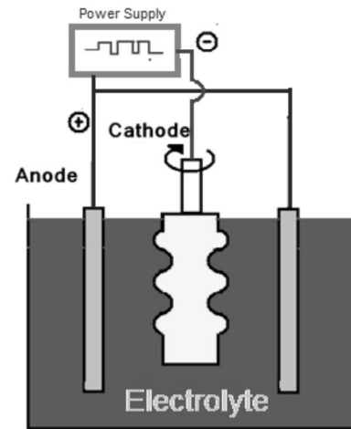
Fig. 1. A schematic diagram of electroforming System
