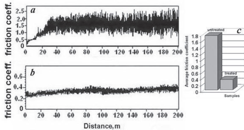
Fig. 3. The friction coefficient factor against sliding distance for (a) untreated and (b)PEN/C treated samples. (c) Average value of friction coefficient factor
