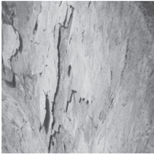
Fig. 2. corrosion products in the interior surface of stack
