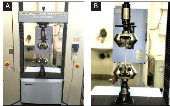
Fig. 4. Tensile Testing Machine (Shimadzu) a) Tensile testing machine (Shimadzu) b) Tensile test specimen loaded in the UTM
