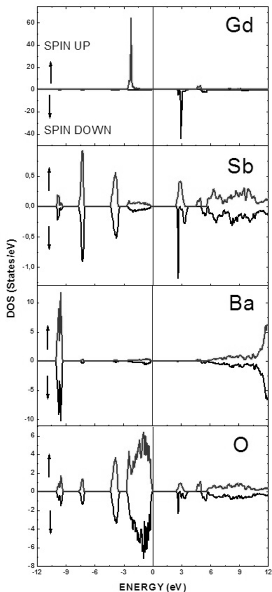
Fig. 6. Partial DOS with spin up and down polarizations for the Ba_2GdSbO_6 double perovskite.
