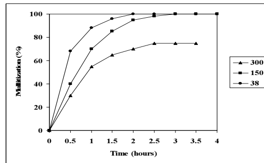
Fig. 7. Evolution of mullitization versus the soaking time at 1550 °C/2h isothermal treatment for kyanite concentrates with different particles size
