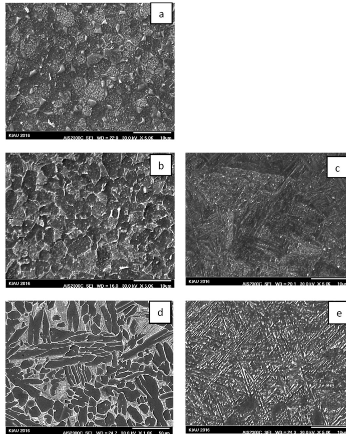
Fig. 1. The microstructure of the heat treated samples. a) As-received sample b) 930A550 c) 930W550 d) 1060A550 and e) 1060W550.
