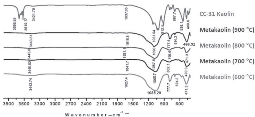
Fig. 4. FTIR spectra of the kaolin and metakaolin calcined at different temperatures.
