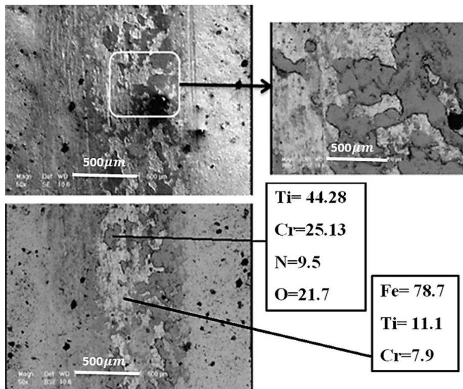
Fig.9. Scanning electron micrographs (SE and BSE) of the wear track in Ti, CrN coatings at sliding distance of 500m.
