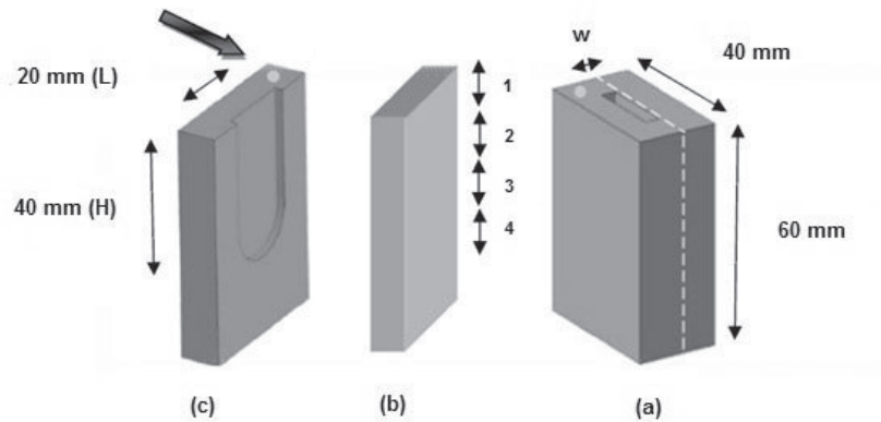
Fig. 1. (a) The sample assembly (b) investigated surface and (c) grooved part.
