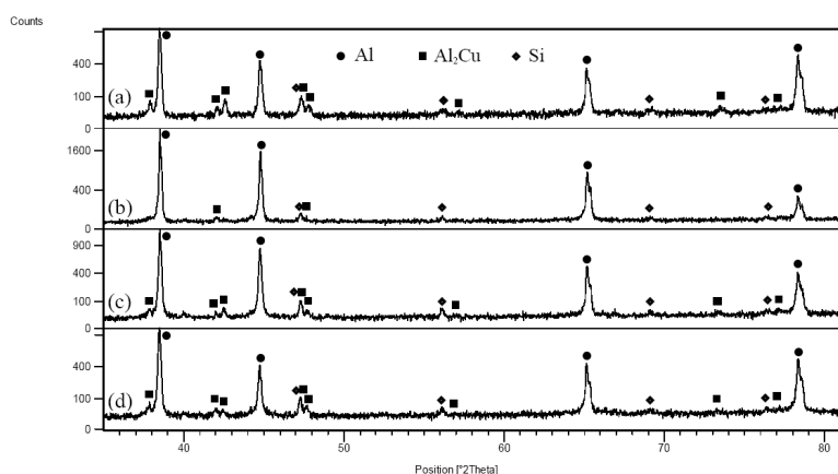
Fig. 3. A comparison between the X-ray diffraction patterns before and after the heat treatment (path 1) in the (a) as-cast sample, (b) 1 hr of aging, (c) 3 hrs of aging and (d) 5 hrs of aging
