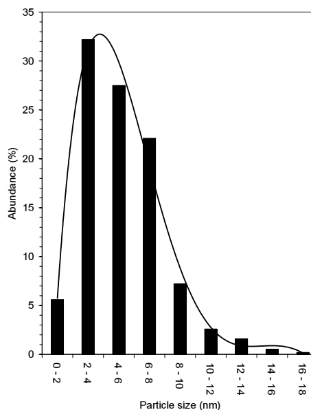
Fig. 2. Transmission electron micrographs recorded from a small region of a drop-coated film of chloroauric acid solution treated with the ethanol extract of black tea (upper left picture) and its tannin fraction (lower left picture) for 15 min (scale bars correspond to 50 nm). The related particle size distribution histograms (right side pictures) obtained after counting 350 individual particles for each sample.
